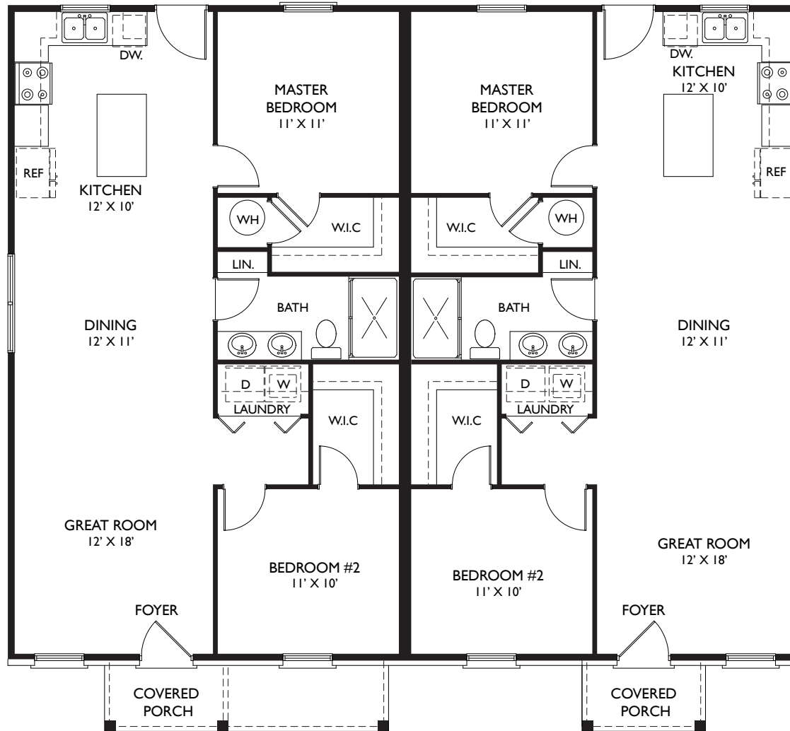
MAIN LEVEL - UNIT 1
