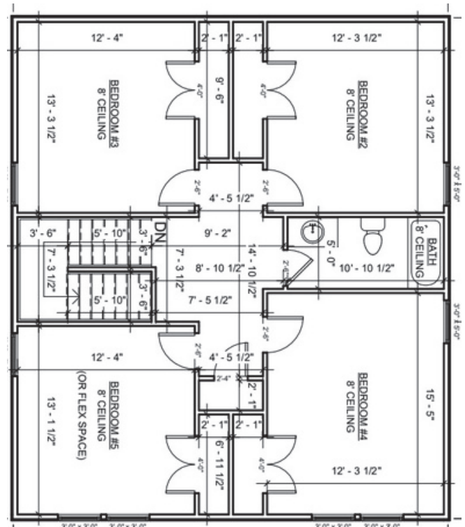
2nd Level
