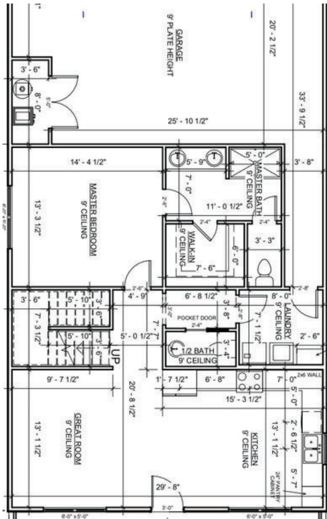
Main Level
