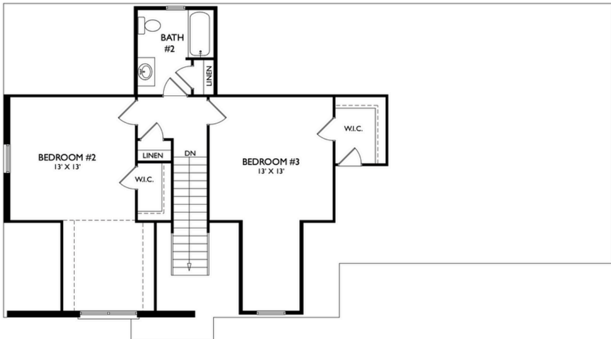
SECOND FLOOR
