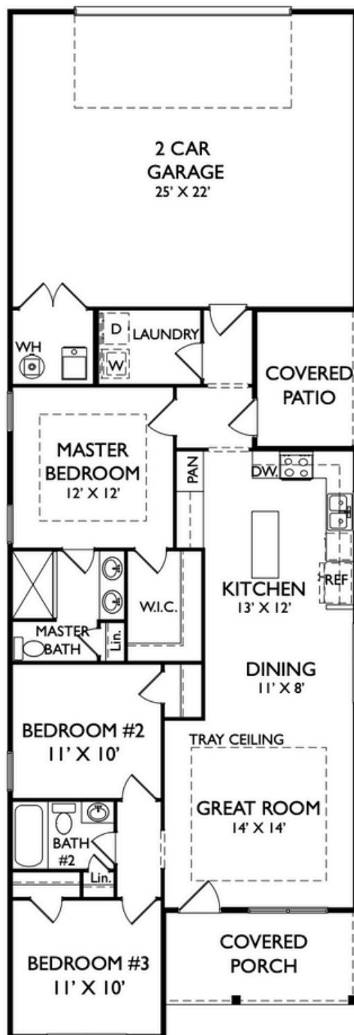
MAIN FLOOR
