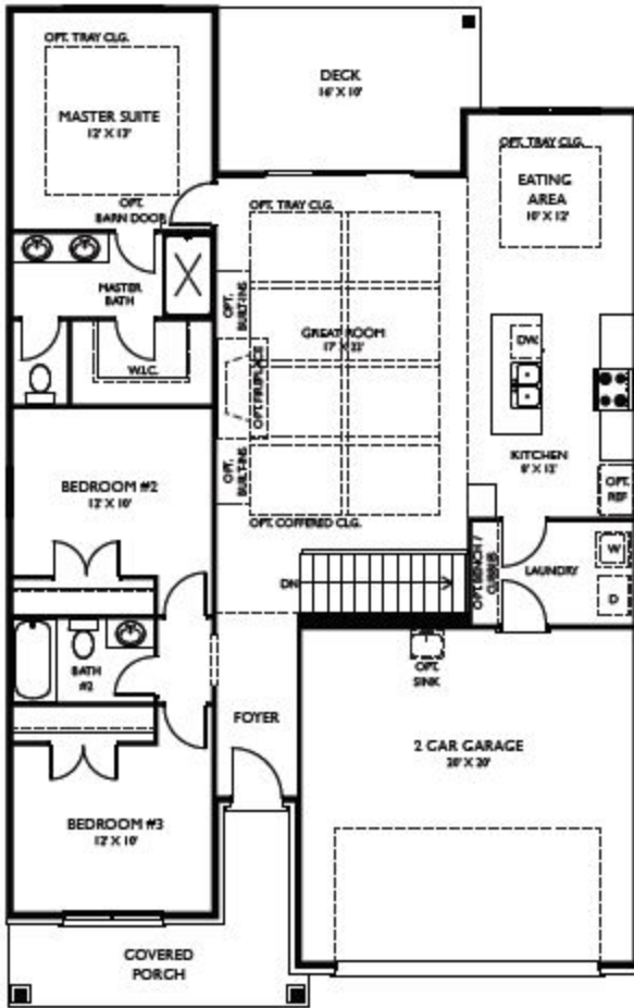
MAIN LEVEL 1,484 SQ.FT.
