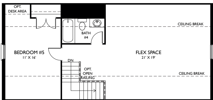
OPTIONAL BONUS ROOM 818 SQ. FT.
